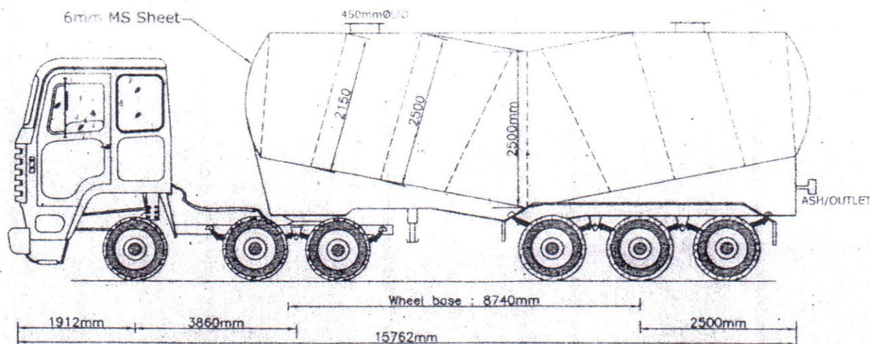
SIDE ELEVATION OF TRACTOR & TRAILER COMBINATION - : AMW 4923TR (202/2011)
