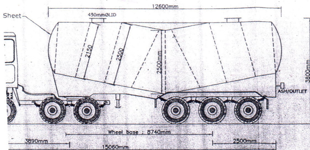
SIDE ELEVATION OF TRACTOR & TRAILER COMBINATION : MAN CLA 49.220(425/2012) : MAN CLA 49.280(94/2007)
