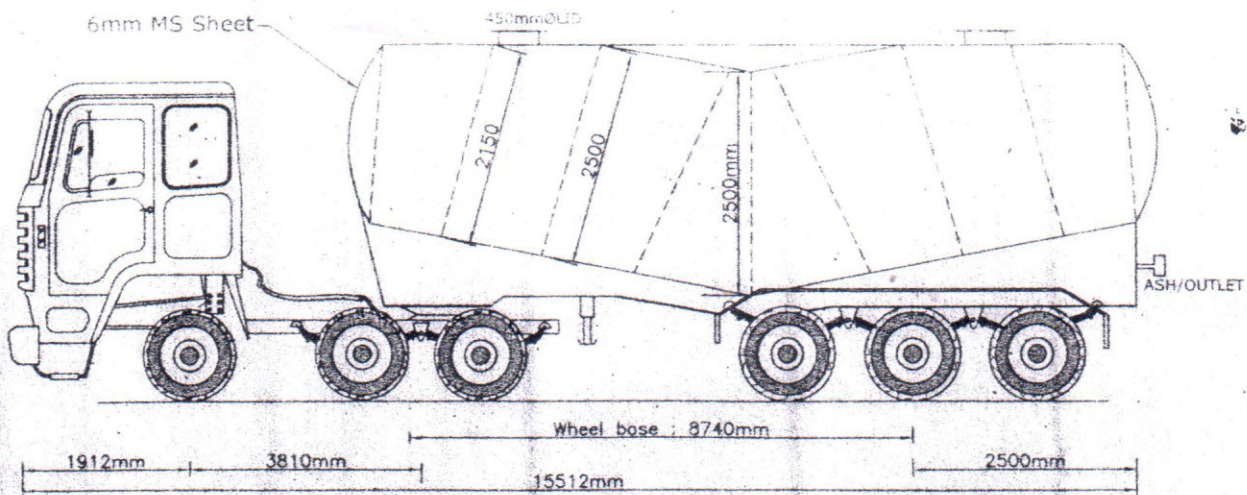
SIDE ELEVATION OF TRACTOR & TRAILER COMBINATION - : AL FV 4923(8/2010)
