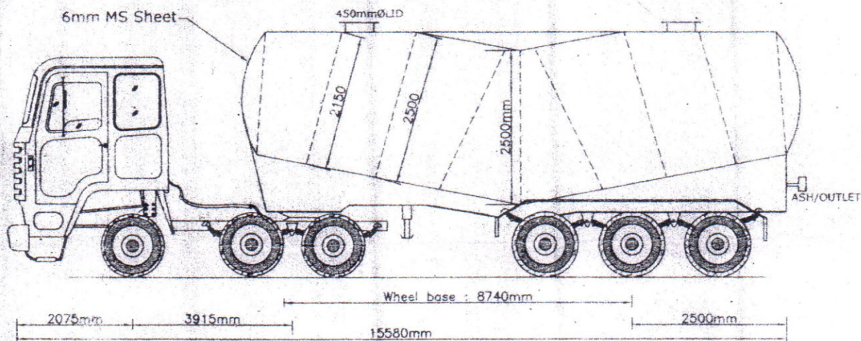
SIDE ELEVATION OF TRACTOR & TRAILER COMBINATION - : TATA PRIMA 49.230 (383/2012) EICHER PRO 8049 (352/2014) TATA PRIMA 4928 S (282/2011)
